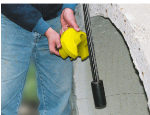
Drop pipe carrier lifting sling through hole in pipe. Align and insert "Tea Cup" pipe carrier into lifting sling.
