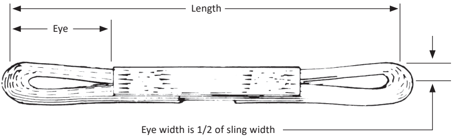
Type RE Reverse Eye Sling
